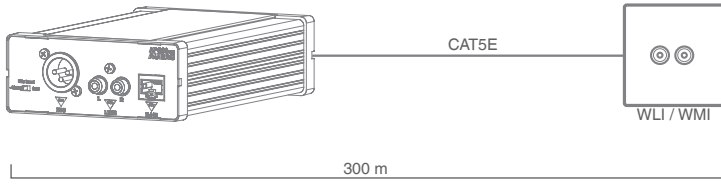
Example 1: One input module connected Maximum cable length: 300 meter
